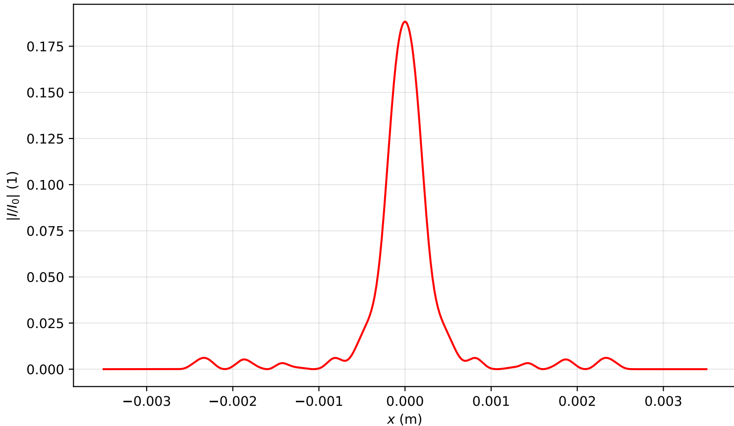
Intensity profile I(x, y = 0, z = 3.025)/I_0 , \text{Pin}=8.0\text{Pcr} , artificial time
